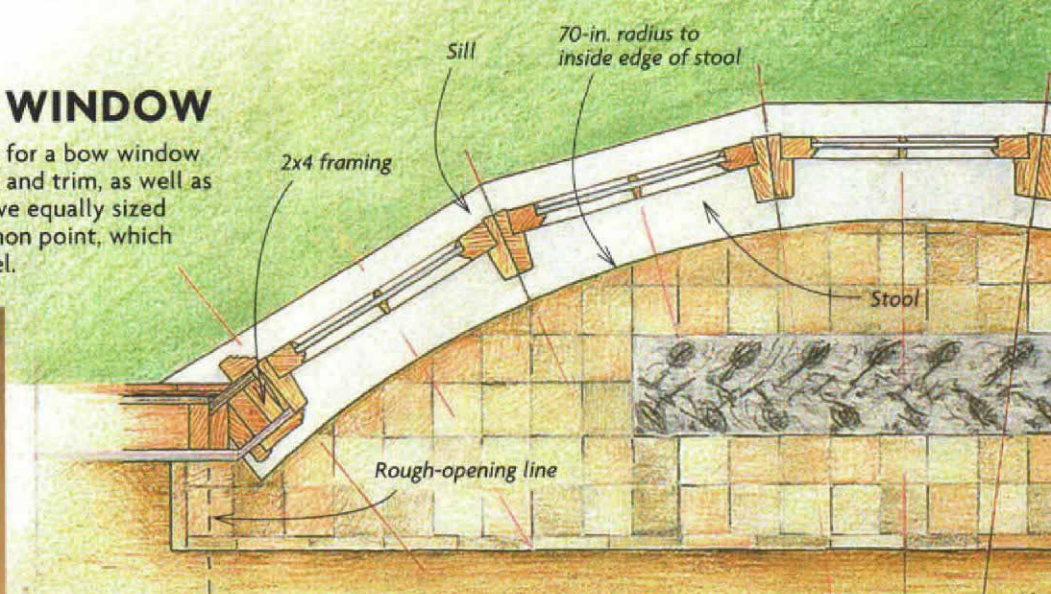
A simple trammel made from scrap helped the author to make an accurate full-scale drawing on 1/4-in. plywood.
