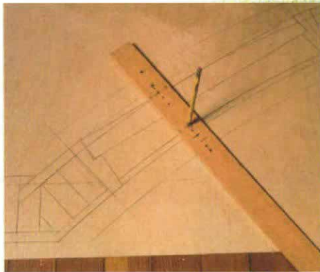
A simple trammel made from scrap helped the author to make an accurate full-scale drawing on 1/4-in. plywood.
